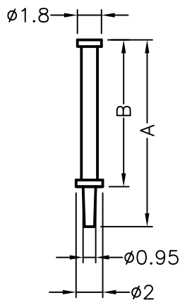
HOLE IN P.C.B \phi 0.95
